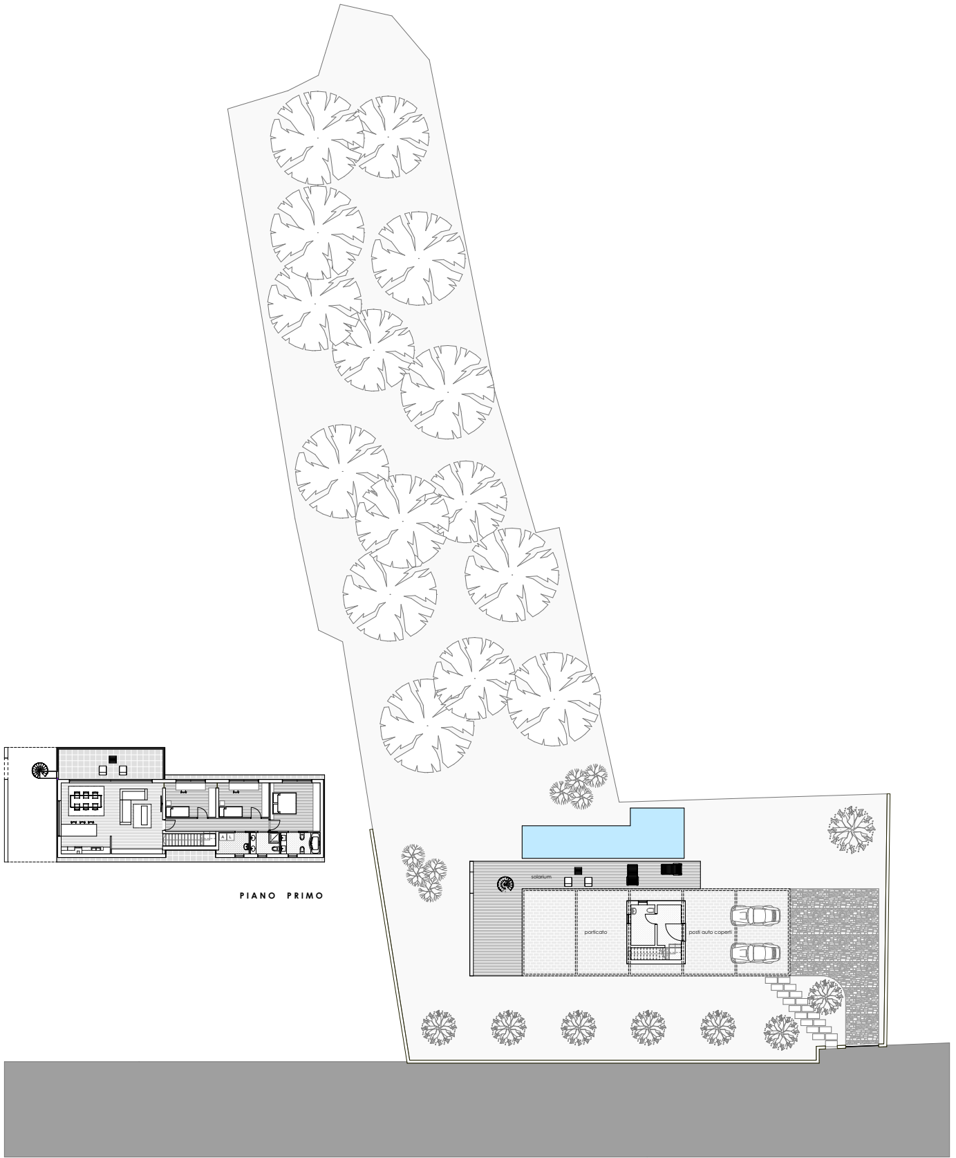
PIANO TERRENO
